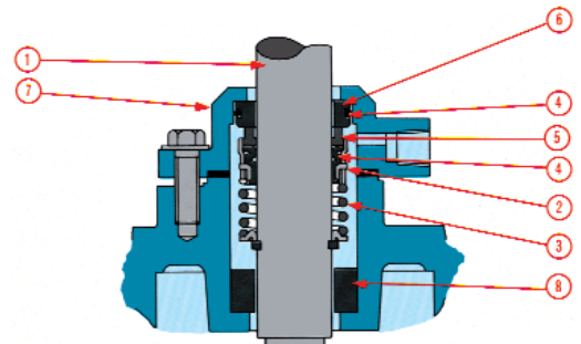
INSIDE UNBALANCED MECHANICAL SEAL ARRANGEMENT
