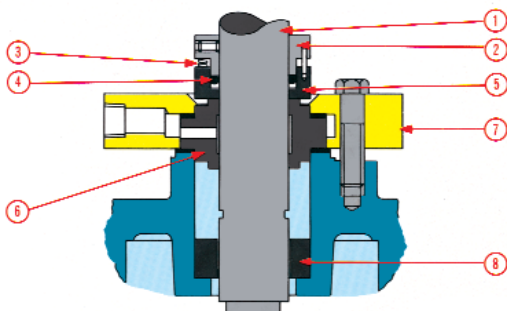
OUTSIDE BALANCED MECHANICAL SEAL ARRANGEMENT
