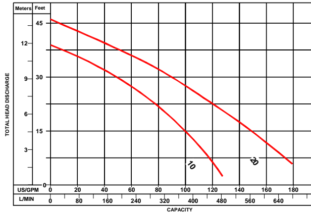
PUMPING CURVE DS & DSK SERIES
