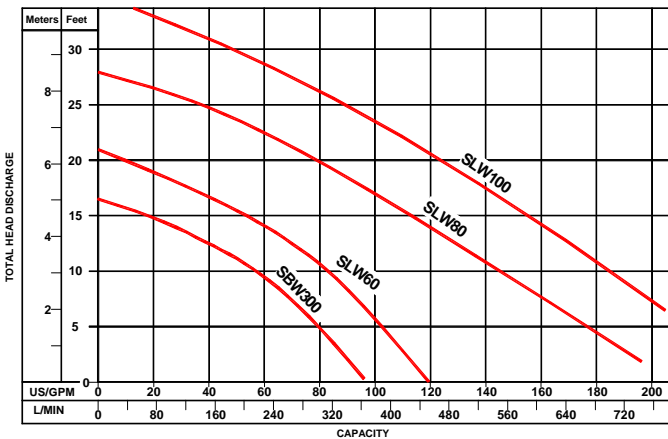
PUMPING CURVES SBW / SLW SERIES
