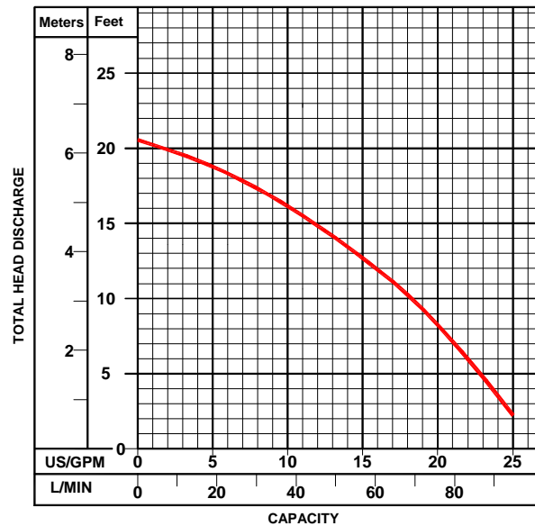
PUMPING CURVE SU180A SERIES
