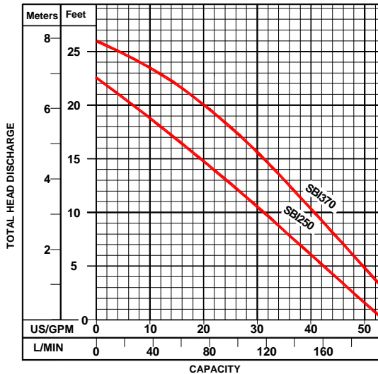
PUMPING CURVES SBI SERIES
