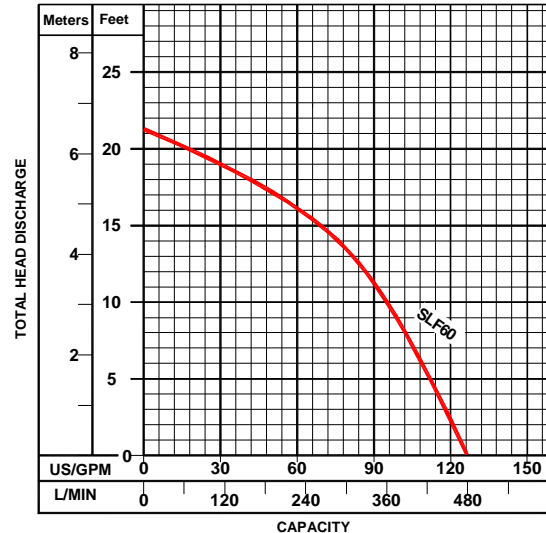
PUMPING CURVE SLF SERIES
